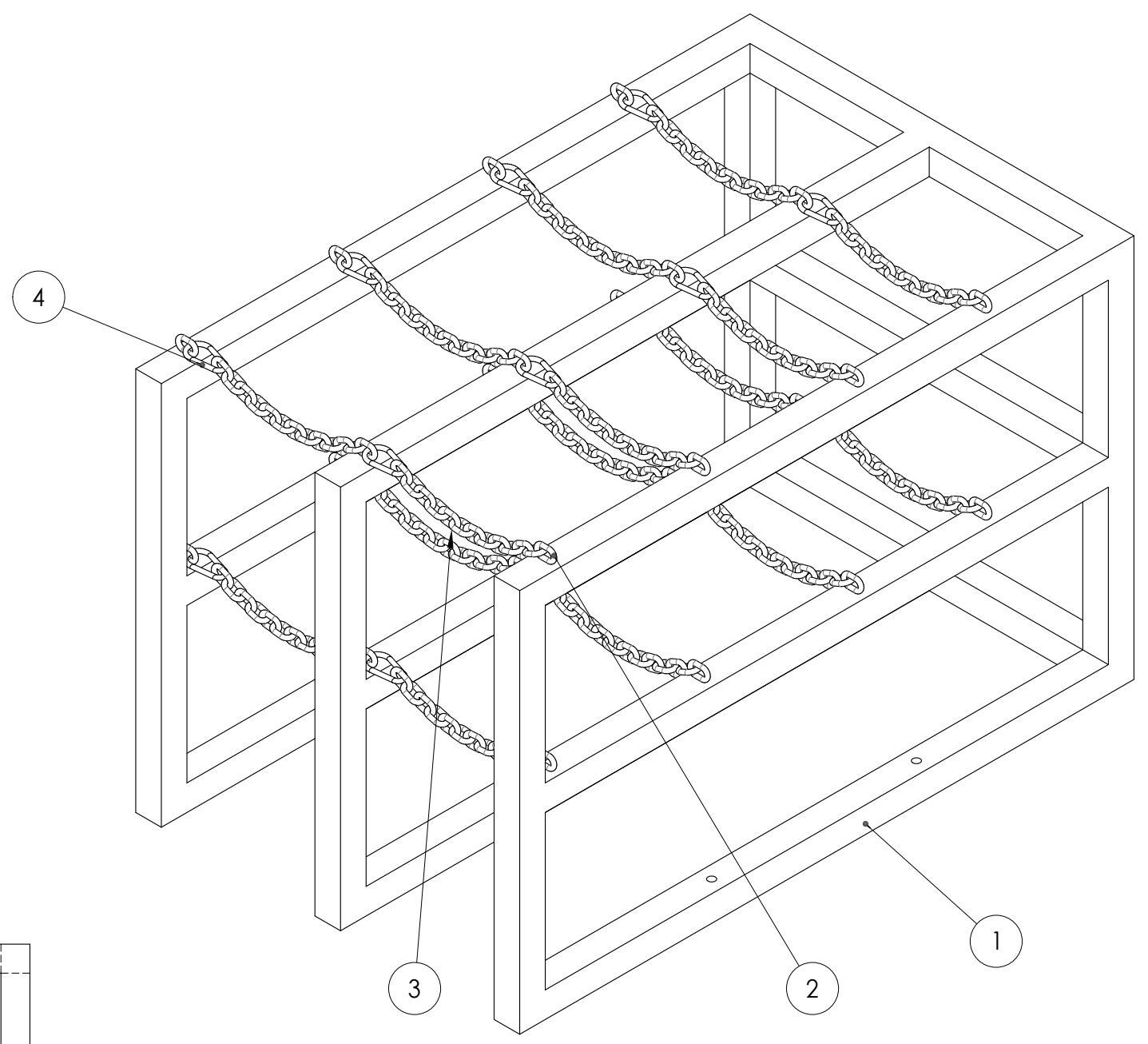
ISOMETRIC SCALE 1:8
