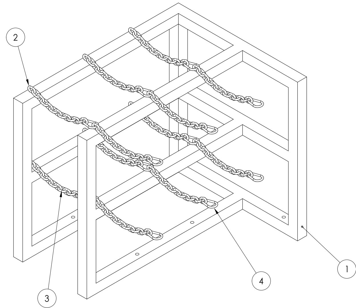
ISOMETRIC SCALE 1:8
